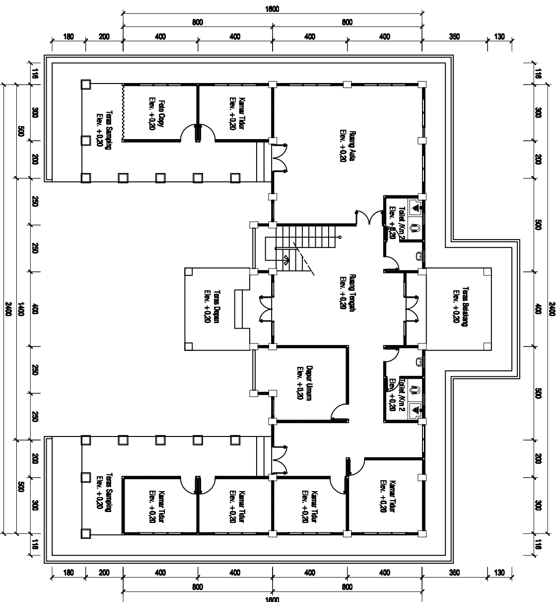
DEWAI LANTAI 1 BAWEAN STUDENT CENTER
